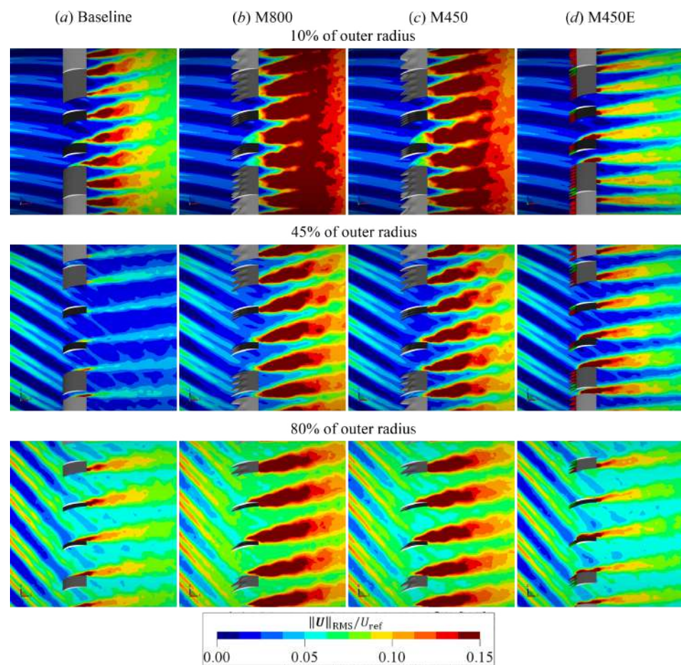
Figure 12. (Side view) Contours of phase-locked standard deviation of velocity magnitude ( \|\mathbf{U}_{\text{RMS}}\| ) at the different radial sections ( top —10%, middle —45%, and bottom —80% of the outer radius) in the fan stage.
