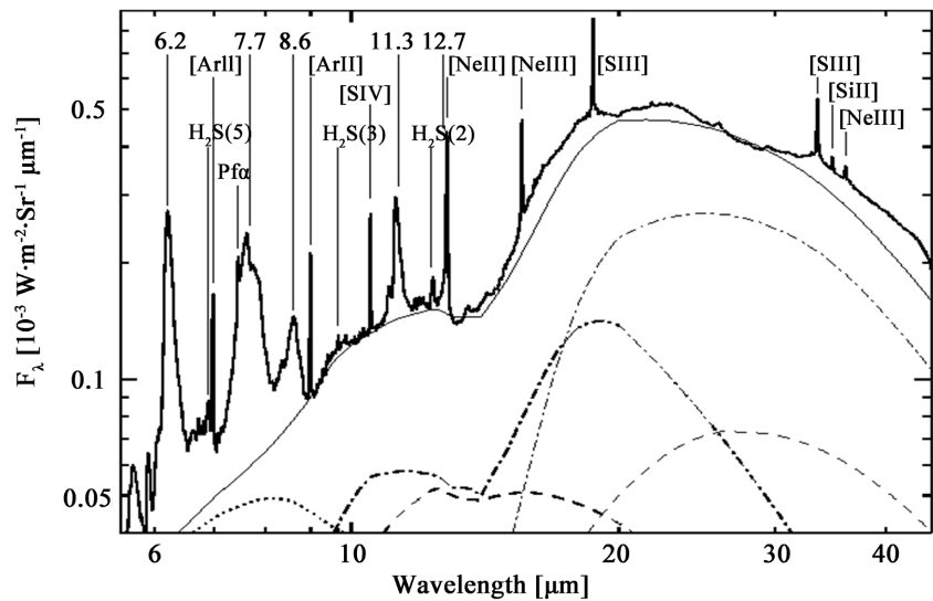
Figure 1. Short Wavelength Spectrometer (SWS) spectrum (full line) in the Orion nebula. The identification of the strongest spectral features (6.2, 7.7, 8.6, 11.3, and 12.7 \mu\text{m} ) is indicated. Adapted from [11].
