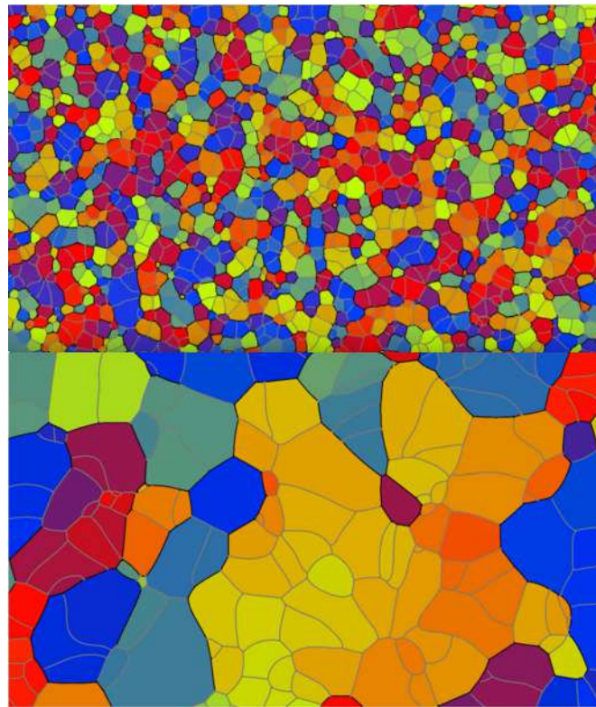
Figure 1. Grain growth process: Changes in connectivity and in cardinality of the system occur. The initial grain structure ( top ) evolves towards the grain structure at a later stage ( bottom ). This grain growth process has been simulated using [65], and a full video of this simulation is available in HD resolution [70].
