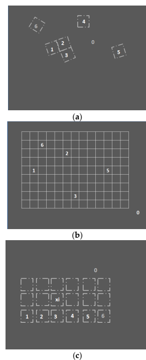
Figure A3. (a) “Molecules” of crystallized space–time forming the initial nucleus for a space–time lattice. (b) Arranged—or by some process self-assembled—cubes in a regular lattice. Their names (indices) are a priori random, and cube #2 does not necessarily have to be a neighbor of cube #1. Note, the volume outside the structured grid is filled by an “unstructured matrix” volume 0, to recover the entire original region of space (dark). (c) In contrast to (b) the cubes—though arranged in a regular lattice—in this situation, are separated by a “foam” of the matrix thing 0. Such a configuration appears quite frequent in nature, e.g., atoms in a crystal being separated by vacuum/fields. In this case, all x_i are connected to the matrix thing only and do not have any direct correlations.
