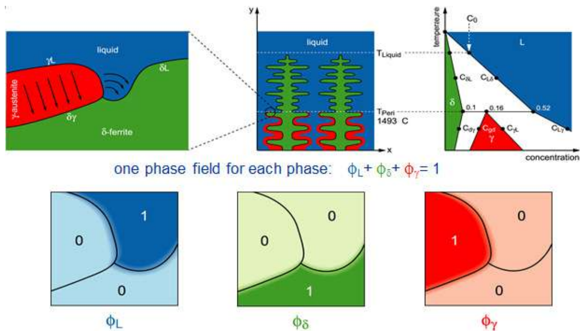
Figure 5. Schematic of a peritectic reaction in a steel grade. Red/green/blue areas indicate regions being occupied by the three phases: austenite ( \gamma ) ferrite ( \delta ) and liquid melt (L). Wherever there is only (!) liquid, no ferrite, and no austenite may be present. The phases pairwise coexist and collocate at their dual boundaries. All three phases coexist and collocate at the triple junction in the middle of each picture. The upper right inset (the phase-diagram) indicates that the phases also coexist in the same energy interval (i.e., at the same temperature). Note the Basic Equation for the three things in the center of the figure.
