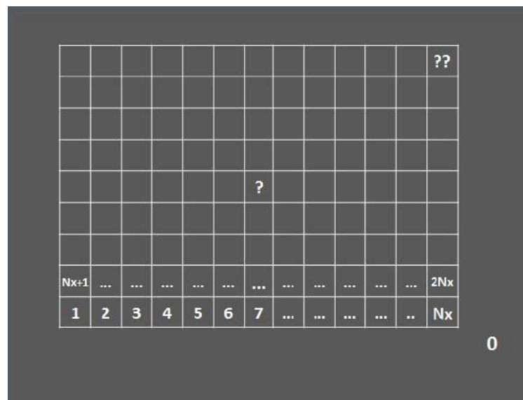
Figure A4. A linear naming scheme can also be extended to 2D and 3D. In this 2D example, N_x is 13 and N_y is 9. The index of cell “?” is 4 \times 13 + 7 = 59 and cell “??” has the value N_x \times N_y = 9 \times 13 = 117 . Cube #5 would obtain cube #18 ( N_x + 5 ) as an additional neighbor (“top”-neighbor) in this 2D example.
