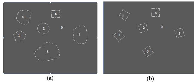
Figure A2. (a) The shape size of the abstract sub-regions a priori is arbitrary. They do not need to be interconnected, regular shaped, or have the same size. Actually, the abstract sub-regions could also be the volumes covered by the different things themselves. (b) As these sub-regions are abstract regions they may be considered as tiny—elementary—cubes, all with the same size. Still, they do not need to be interconnected but might only be embedded in an unstructured matrix 0 (dark). They may reveal different orientations.
