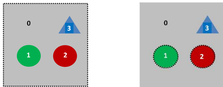
Figure 13. The “universe individual” (left, marked by its dashed boundary) is one of the possible selections for an underlap of the two things 1 and 2, as per the definition of the universe hasPart of all things. Another possible selection is the mereological sum representing the minimum object comprising both things (right, boundaries also marked by dashed lines).
