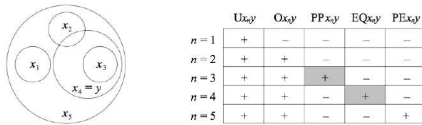
Figure 12. Overview of mereological relations (underlap, overlap, proper parthood equality, and enclosure) between different things. [ https://plato.stanford.edu/entries/mereology/ (accessed on 1 November 2021)].
