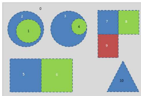
Figure 16. Different configurations of things forming a variety of interfaces, triple lines, and quadruple points. The total boundary of thing 7 \partial\Phi_7 , consists of boundary regions with the matrix 0, and with things 8 and 9 and also includes triple and quadruple junctions, meaning, \partial\Phi_7 = \partial\Phi_{7,0} + \partial\Phi_{7,8} + \partial\Phi_{7,9} + \partial\Phi_{7,8,0} + \partial\Phi_{7,9,0} + \partial\Phi_{7,9,8,0} (see text for the other objects).
