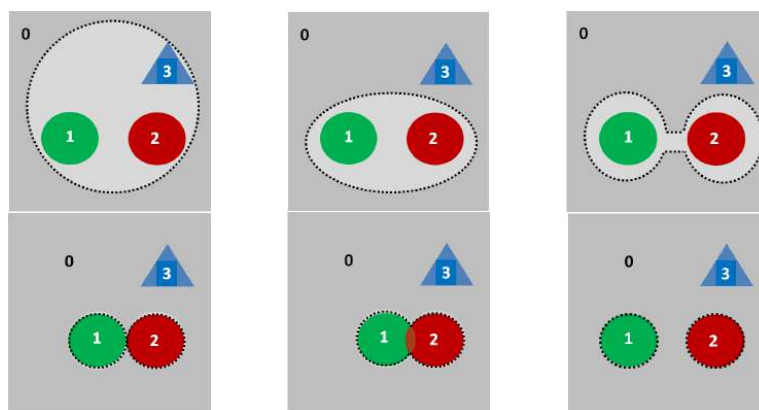
Figure 14. Different possible underlaps (light grey) for two things (1/green, 2/red) as part of a universe individual (dark grey) having three things (1, 2, and 3) and a matrix thing (0) as parts. Note that the underlap in all cases, except for the lower-right case, is a single, self-connected object. The lower-right case corresponds to the mereological sum of two disconnected things. Even for disconnected things the underlap may however be self-connected (see text). The different possible self-connected underlaps depicted in this figure differ in their size and thus allow for a continuous description of a transition from “isDisconnected” via “isExternalContact” to “isPartOf” with a variable describing this transition being the “fraction” the underlap takes of the universe (see text). The mereological sum of two disconnected parts does not fit into such a sequence, as its self is not self-connected. The mereological sum of two connected parts, in contrast, fits well into the sequence, as it is a self-connected object.
