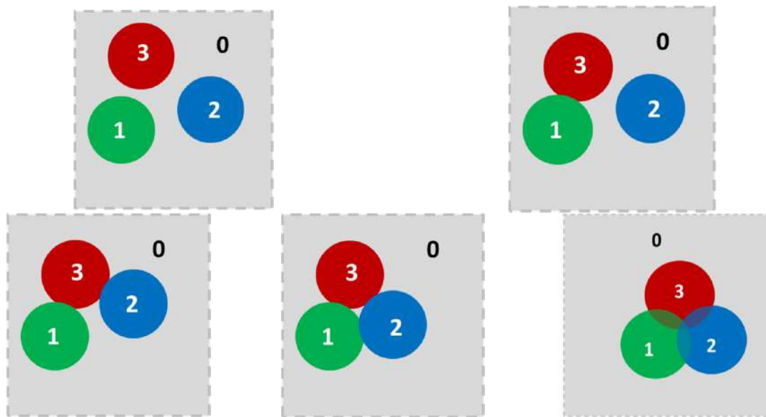
Figure 7. Multiple things in a volume. Two configurations ( top ) can be well described by classical mereotopology. Top left: All things are mutually disconnected resp. connected with the matrix only. Top right: 1 isPartOf 3, 2 isDisconnected from both 1 and 3. Three configurations typically are not described by classical mereotopology ( bottom ). They differ in number and type of triple junctions. This number increases from 4 ( bottom left ) to 6 ( bottom middle ) all of which include the matrix thing. Eventually ( bottom right ), a situation of 4 triple junctions is possible, in which one of these triple junctions does not comprise the matrix thing. Note that the number of triple junctions is always even. The case of “external contact” seemingly having only one triple junction is discussed separately (see text).
