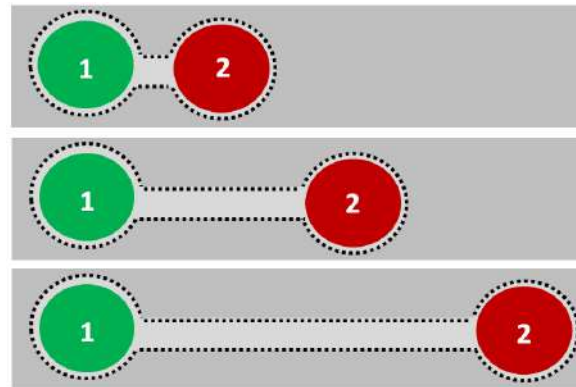
Figure 15. Schematic sketch of two things being separated by different “distances” (increasing from top to bottom). While the boundary between most of part 1 and the underlap and most of part 2 of the underlap is minimized and will essentially not depend on their relative position, the volume of a connecting “string”, “tube”, or “path” will, essentially, linearly depend on the distance.
