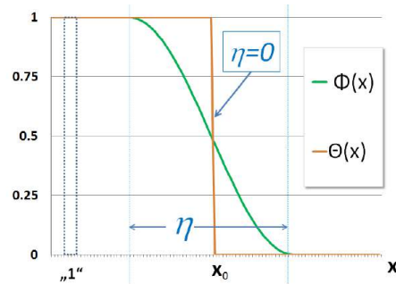
Figure 3. Schematic view of the phase-field function \Phi(x) . This function takes a non-zero value wherever the object is present; it takes exactly the value 1, where it is the only present object and is 0 elsewhere (i.e., where the object is absent). It exhibits a continuous transition between two regions over a finite interface thickness \eta . The Heaviside function \Theta(x_0) , characterized by a mathematically sharp transition at x_0 , is shown as a reference. The dotted region “1” on the x-axis, exemplarily corresponds to the tiny volume “1” in Figure 2b, where only the solid is present.
