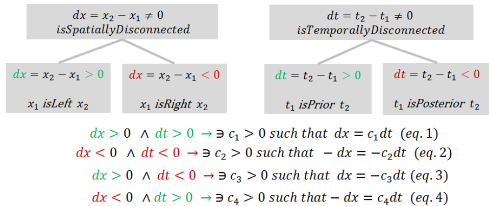
Figure 20. The c_i in the different equations a priori are not necessarily identical. Requesting invariance under parity operations ( P(x) = -x ) and under time inversal symmetry operations ( T(t) = -t ), however, limits their choice. Applying the parity operation on Equation (1) leads to Equation (4) if c_1 = c_4 , applying it to Equation (2) leads to Equation (3) if c_2 = c_3 . Applying the time inversal operation to Equation (2) leads to Equation (4) if c_2 = c_4 . Eventually, applying it to Equation (3) leads to Equation (1) if c_3 = c_1 . The request for satisfying invariance under both of these operations thus leads to c_1 = c_2 = c_3 = c_4 = c .
