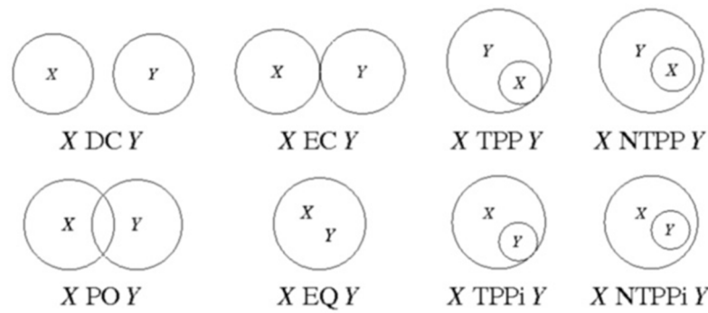
Figure 11. Region connection calculus ( https://en.wikipedia.org/wiki/Region_connection_calculus (accessed on 1 November 2021)). Disconnected (DC), externally connected (EC), tangential proper part (TPP), non-tangential proper part (NTPP), partially overlapping (PO), equal (EQ), tangential proper part inverse (TPPi), and non-tangential proper part inverse (NTPPi).
