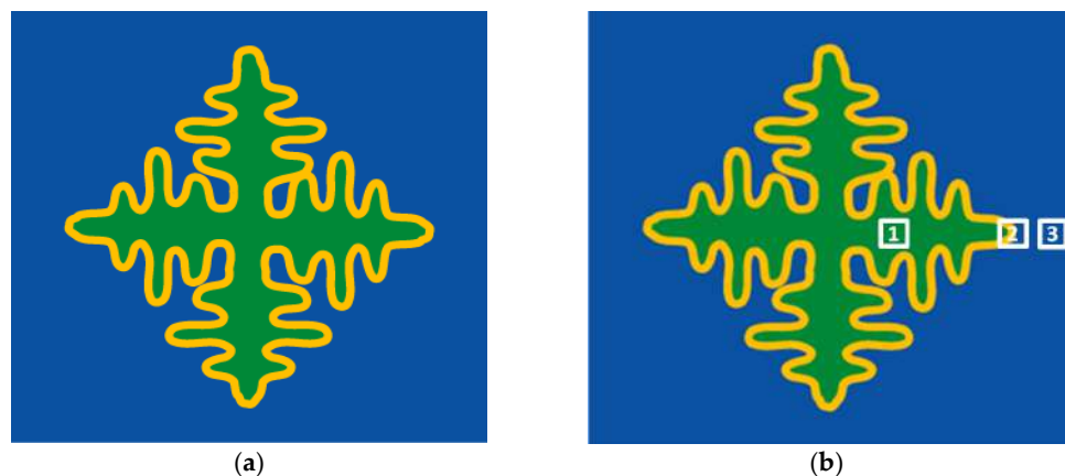
Figure 2. (a): A solid phase \Phi_s (green center region) coexisting with a liquid phase \Phi_l (blue outer region) in a volume. The fraction solid \Phi_s amounts to approx. 1/3 of the overall volume, while the fraction liquid is approx. 2/3 . Both are non-zero and their correlation (yellow) thus exists as a boundary in the overall volume. Nothing can however be said about the position of this boundary without further discretization of the volume (Figure 2b). (b): In above tiny volume “1”, the fraction solid \Phi_s amounts to exactly 1, while the fraction liquid \Phi_l is exactly 0. In the tiny volume “3”, the fraction solid \Phi_s amounts to exactly 0, while the fraction liquid \Phi_l is exactly 1. In contrast, both fractions are non-zero and their correlation (yellow) exists in the tiny volume “2”, which thus comprises a boundary.
