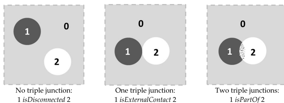
Figure 6. Classification of different configurations known from mereotopology and region connect calculus according to the number of triple junctions present in the system. Dyadic relations between two things turn into triadic relations of three things if the matrix thing (0) is taken into account.
