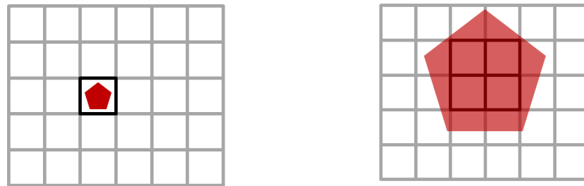
Figure A5. Left: If \Phi (red) is ProperPart of a specific volume element x_j (depicted by the black boundary) this particular volume element defines the position of \Phi up to some remaining uncertainty. Right: All volume elements x_j , being parts of \Phi , denote regions where \Phi is present. If they are ProperParts of \Phi , there is no other thing present in this particular volume element.
