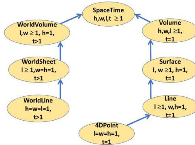
Figure A1. Concept to integrate different 4D objects (“points”, “lines”, and “surfaces”) as subclasses of a 4D physical space–time. The classes are differentiated by the values of the variables l, w, h, and t (see text). Arrows are to be read as “isPartOf” relations.
