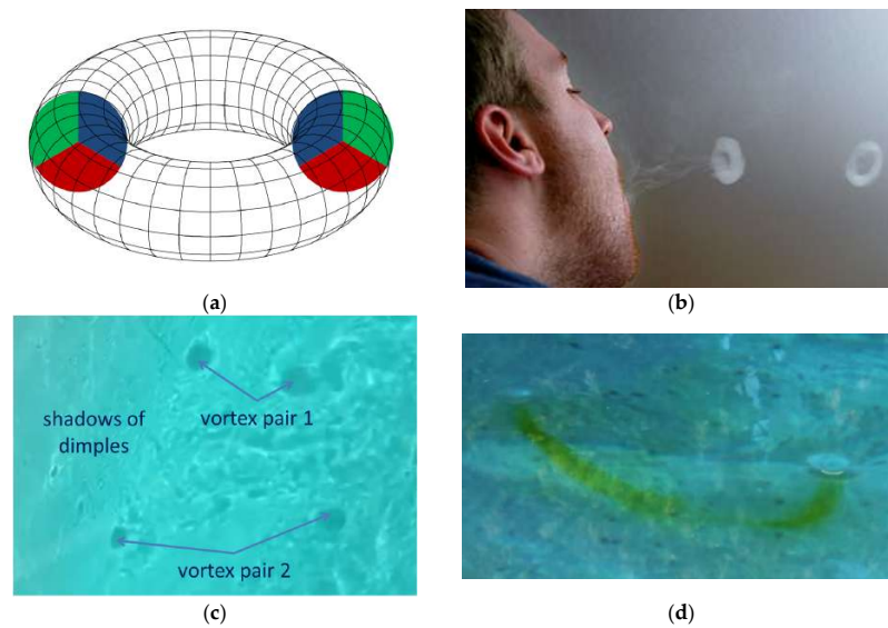
Figure 9. (a) Visualization of a vortex resp. of a torus. A 2D section reveals two vortices with opposite helicities. (b) Smoke vortices as propagating objects in a 3D world. Photo reproduced from [79]. (c) Triple junctions in a 2D section at the water surface always show up as pairs, shown here for two flow vortices (“dimples”) in a pool—so-called Falaco solitons [80]. “Falaco solitons appear to have properties claimed by the String theorists trying to explain Quantum Gravity” [81]. (d) Experimental visualization of 3D connectivity of two vortices [82]. The surface dimples have been colored with green fluid, which reveals them being coupled in the third dimension in a semi vortex extending under the water surface.
